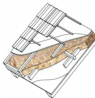
roof
