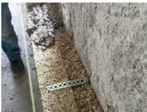
Counterwall of Blocco Ambiente ® with a cavity filled with Bio Beton ®200 Pronto
